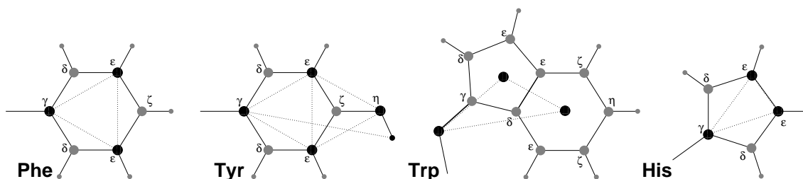
Figure 6.10: The different types of virtual site constructions used for aromatic residues. The atoms used in the construction of the virtual site(s) are depicted as black circles, virtual sites as gray ones. Hydrogens are smaller than heavy atoms. A: phenylalanine; B: tyrosine (note that the hydroxyl hydrogen is not a virtual site); C: tryptophan; D: histidine.
