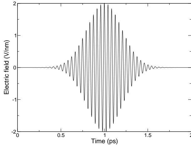
Figure 6.7: A simulated laser pulse in GROMACS.
