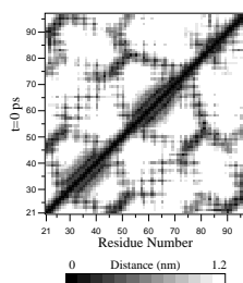
Figure 8.7: A minimum distance matrix for a peptide [165].
