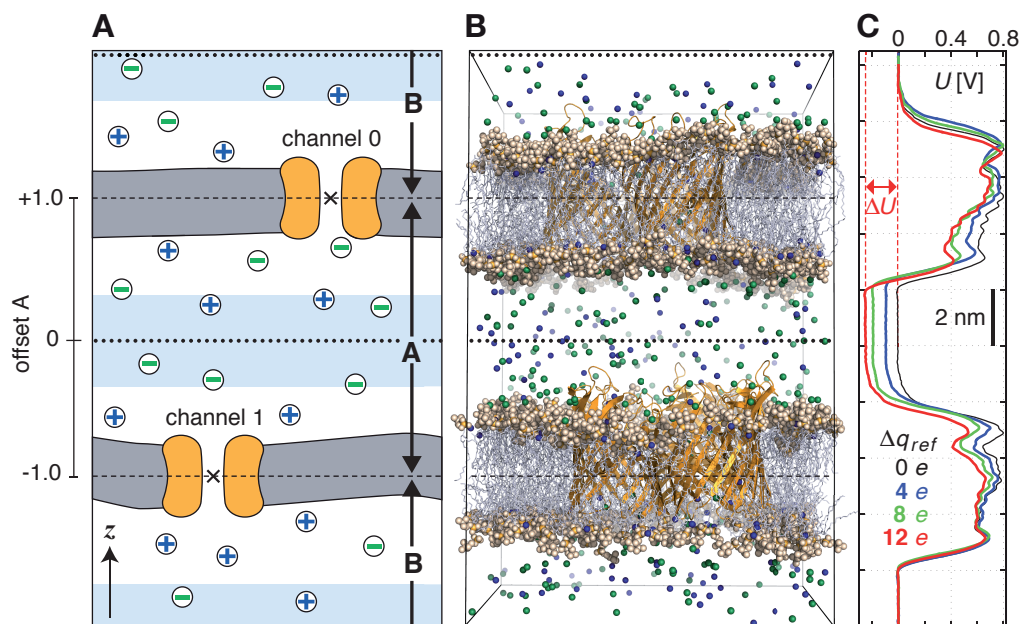
Figure 6.8: Typical double-membrane setup for CompEL simulations (A, B). Ion/water molecule exchanges will be performed as needed between the two light blue volumes around the dotted black lines (A). Plot (C) shows the potential difference \Delta U resulting from the selected charge imbalance \Delta q_{ref} between the compartments.
